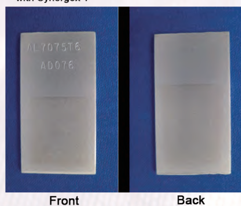
Figure 2—Aluminum 7075 synthetic fluid with Synergex T
