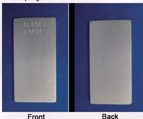
Figure 1—Aluminum 6061 synthetic fluid with Synergex T
